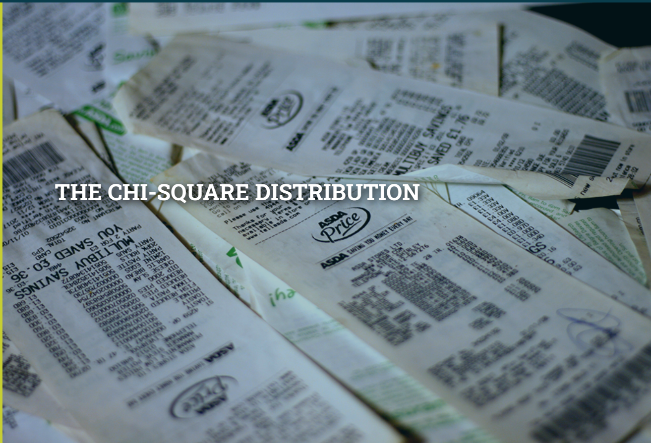
Figure 11.1 The chi-square distribution can be used to find relationships between two things, like grocery prices at different stores. (credit: modification of work “The first few times I used my Asda 'bag for life' I left the receipts in the bottom of the bag” by Pete/ Flickr, Public domain)
