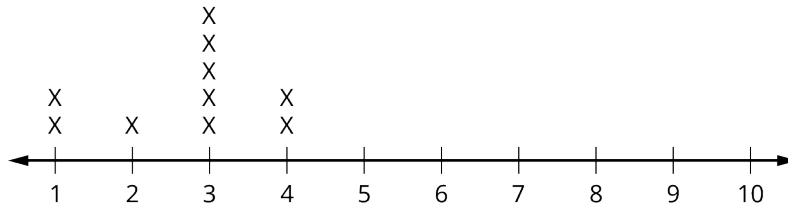
Figure 2.20 Davi's distribution has a left (negative) skew
